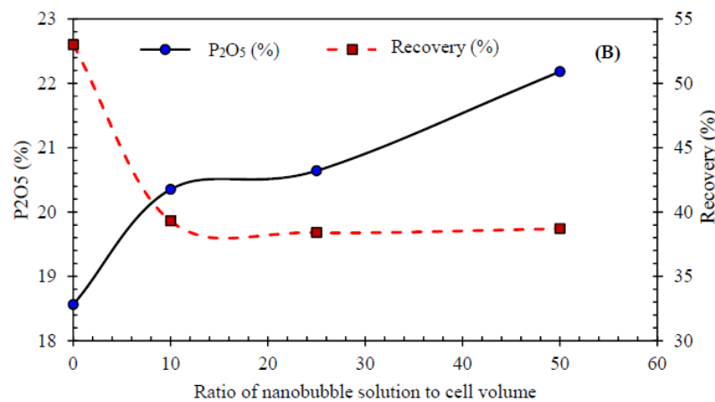
Fig. 8. Effect of nanobubble solution to cell volume ratio in flotation of desliming cyclone overflow (sample B)
