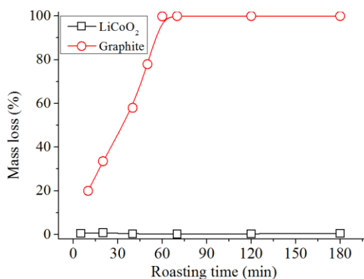
Fig. 4. Mass loss of electrode materials under different roasting time
