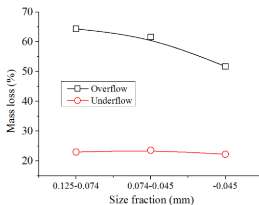
Fig. 7. Separation performance difference of narrow size fraction
