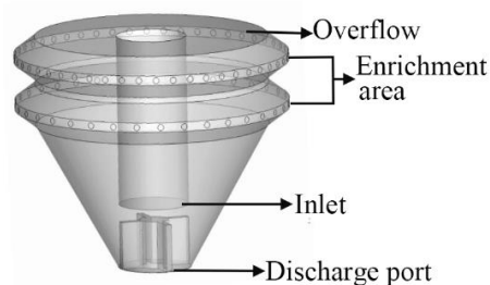
Fig. 3. Structure of the Falcon concentrator
