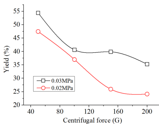
Fig. 5. Influence of centrifugal force and fluidization water pressure on the yield of overflow
