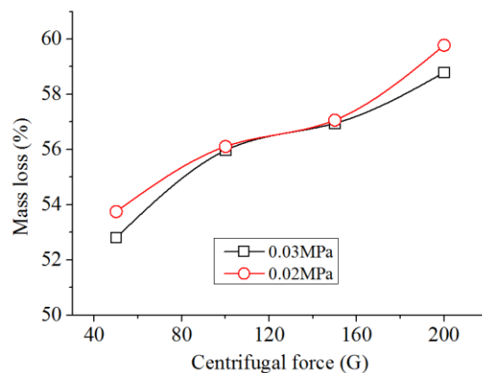
Fig. 6. Influence of centrifugal force and fluidization water pressure on the mass loss of overflow.
