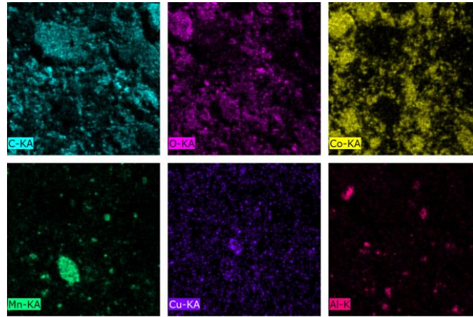
Fig. 2. Surface element distribution of Fig. 1(a)
