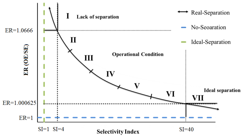
Fig. 6. New upgrading curve based on efficiency ratio (ER) as a function of selectivity index (SI)
