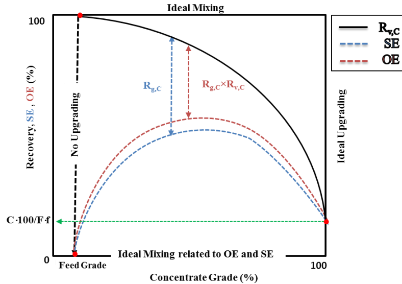
Fig. 3. New upgrading curve based on R, SE and OE as a function of concentrate grade
