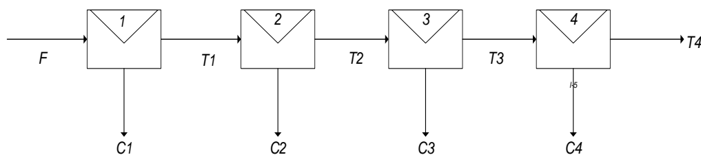
Fig. 2. Flowsheet of galena flotation process
