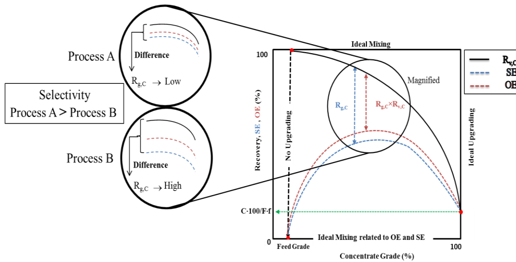
Fig 7. Determination of process selectivity via new upgrading curve and ER index
