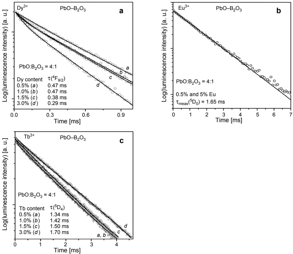
Fig. 4. Luminescence decay curves for \text{Dy}^{3+} (a), \text{Eu}^{3+} (b) and \text{Tb}^{3+} (c) ions in lead borate glasses.
