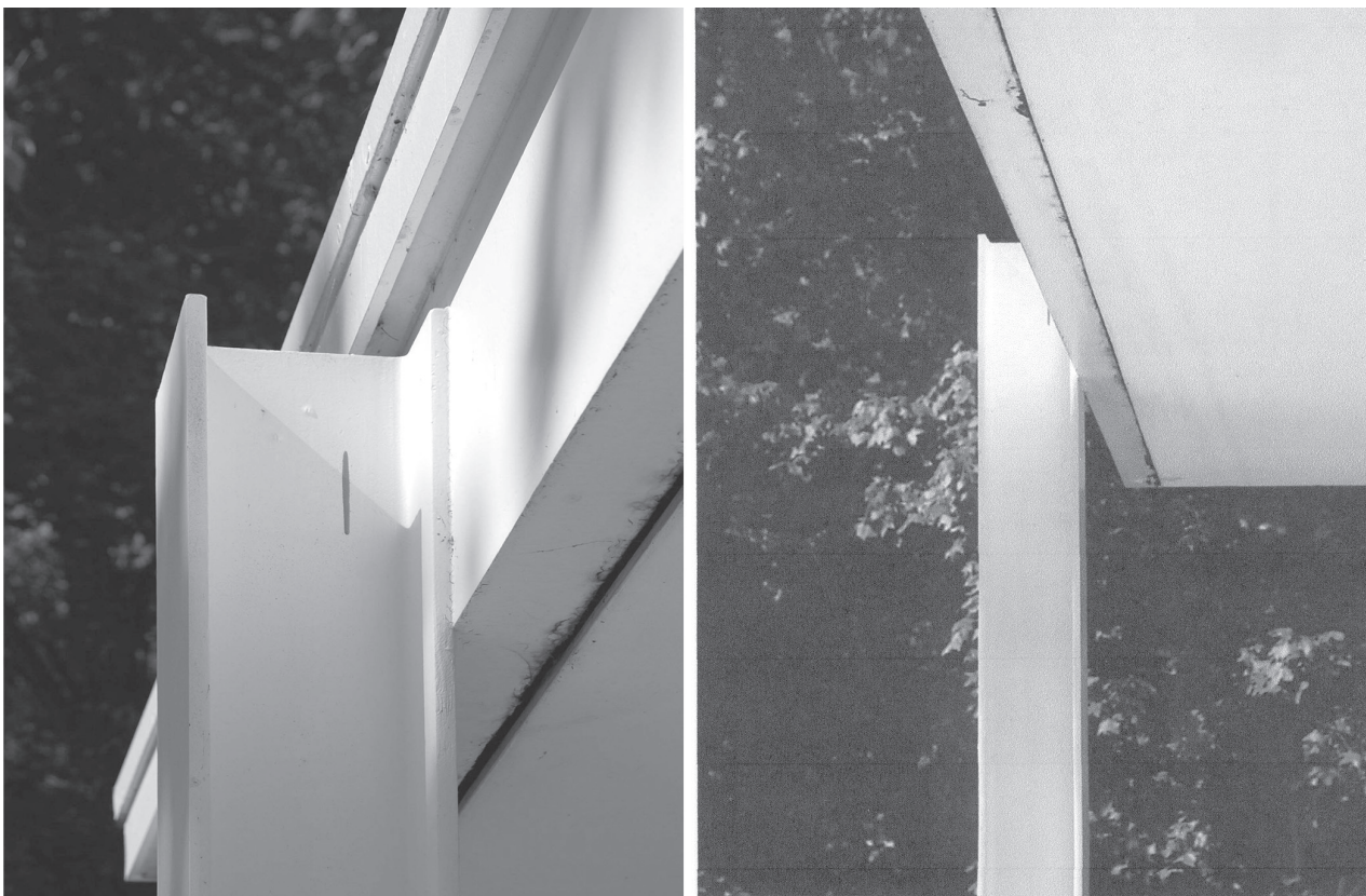
Fig. 13. The tangent union between column and beam in Farnsworth House (photo by A. Cervilla García, September 2012)
