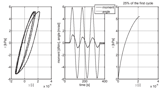
Figure 8: The results of the TS test of sample S3935.
