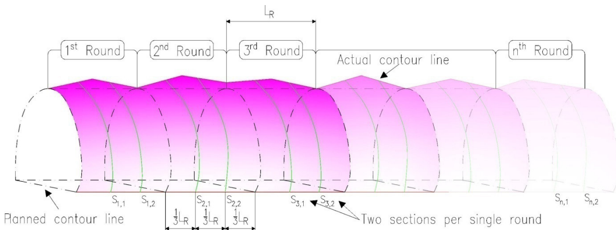
Figure 2: Spacing of measurement sections within a single blasting round [1].
