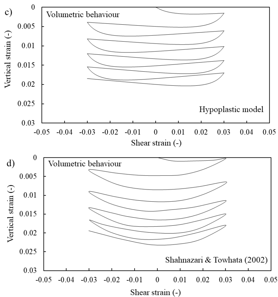
Figure A1: Comparison of a cyclic simple shear test simulated by the hypoplastic sand model and compared with experimental data from literature (Shahnazari & Towhata, 2002): a) stress–strain behaviour (simulation), b) stress–strain behaviour (experiment), c) volumetric response (simulation), d) volumetric response (experiment).
