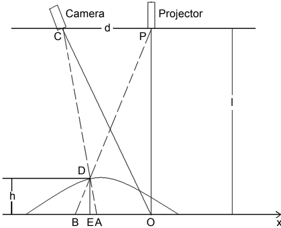
Fig. 1. Optical path of phase measuring profilometry (see text for explanation).
