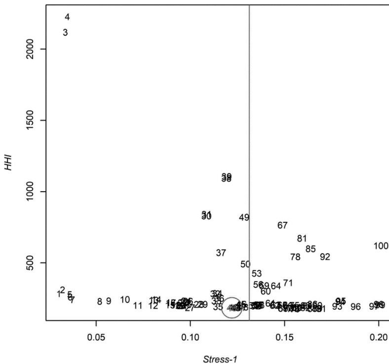
Fig. 1. Stress-1_p fit function values and HHI_p index values for p multidimensional scaling procedures
