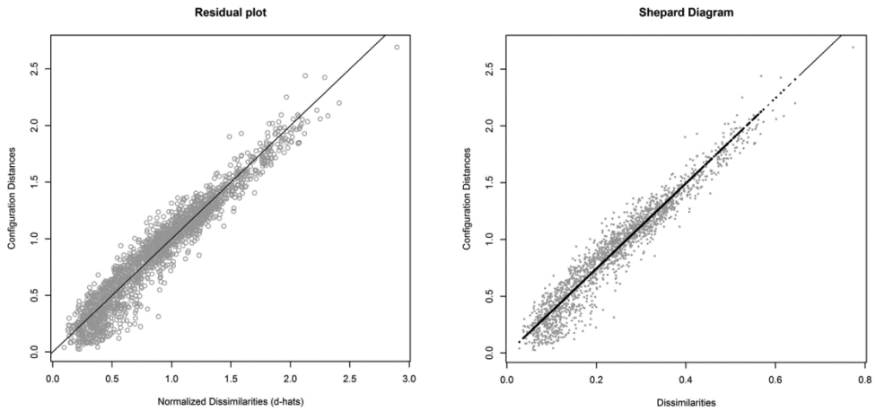
Fig. 2. Residual plot and Shepard diagram
